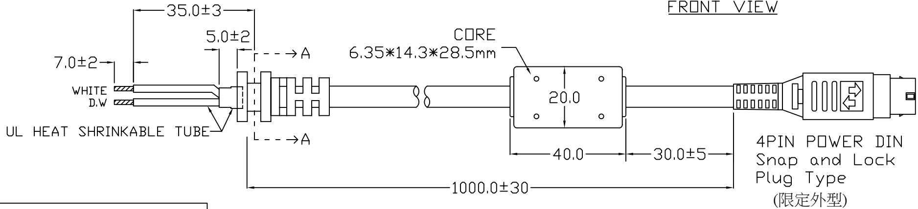
[1571#14AWG 1C+1] SECTIONAL DRAWING
