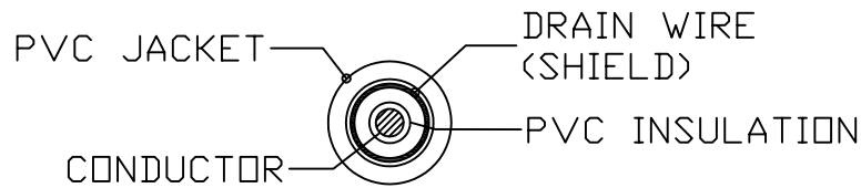
[1571#14AWG 1C+1] SECTIONAL DRAWING
