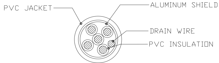
[2464#16AWG 5C+1] SECTIONAL DRAWING
