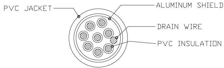
[2464#16AWG 8C+1] SECTIONAL DRAWING
