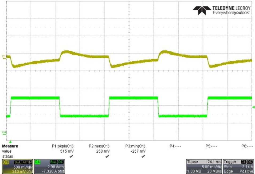
25% to 50% load; 230Vac input
