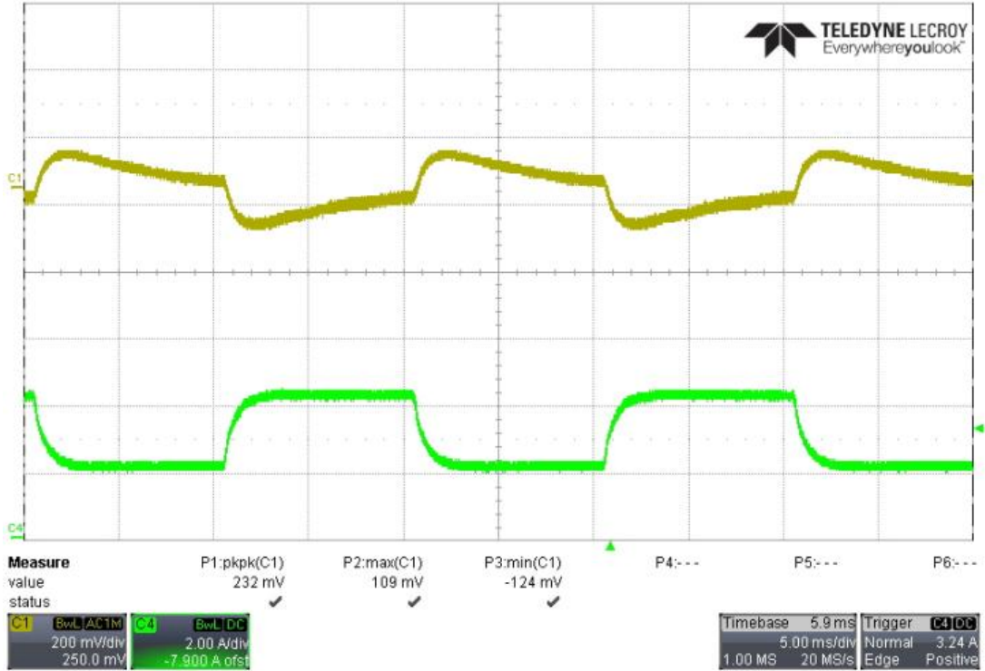
25% to 50% load; with 3950uF capacitance; 115Vac input
