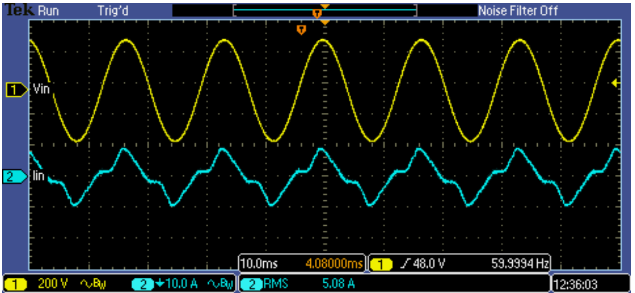
Iin: 10A/div Vin: 200V/div 10ms/div Input Current (100% Load, 220VAC Input)
