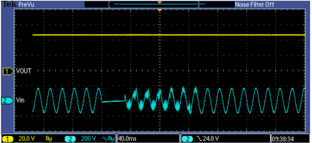
Vin: 200V/div Vout: 20V/div 40ms/div Vin: 110VAC - 32mS Dropout (100% Load)
