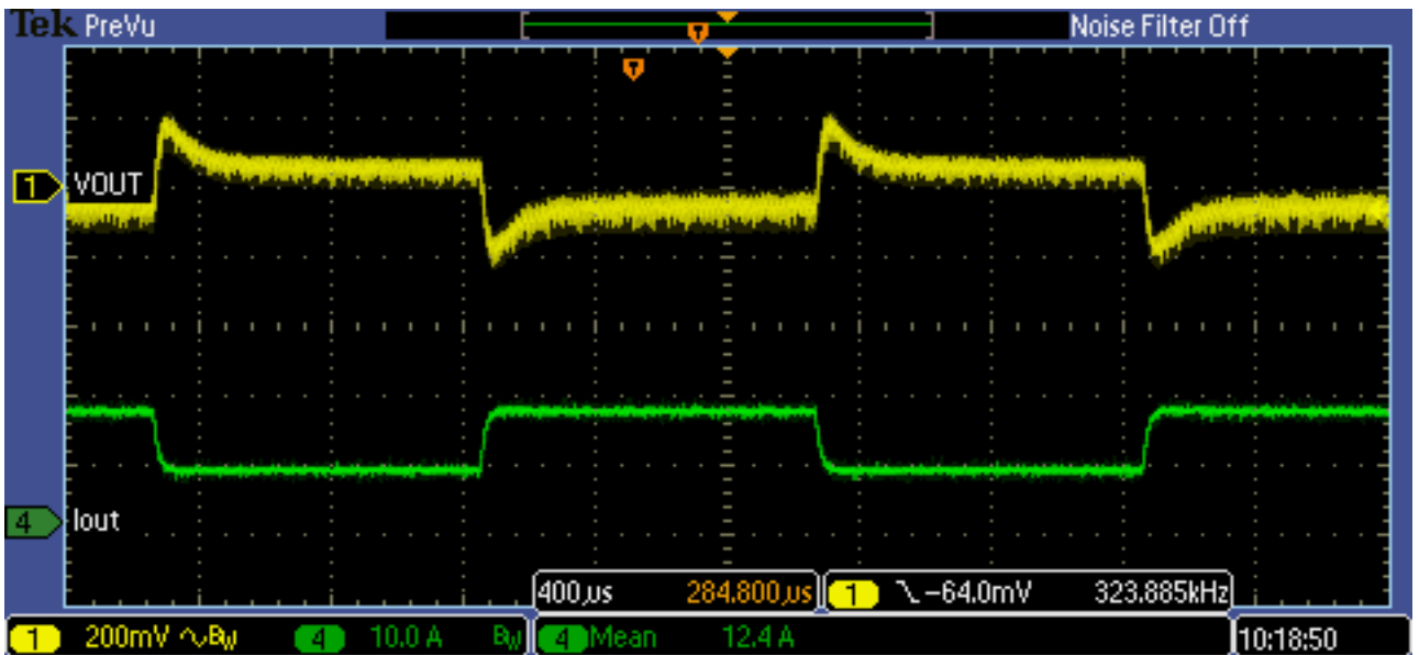
Iout: 10A/div Vout: 200mV/div 400us/div Dynamic Load Response (50% to 100% Load, 220Vac input)
