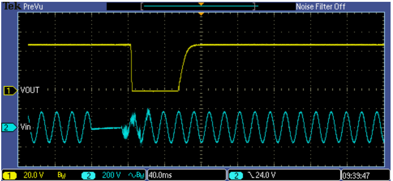
Vin: 200V/div Vout: 20V/div 40ms/div Vin: 110VAC - 33mS Dropout (100% Load)
