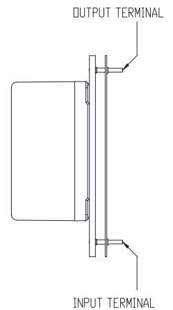
MOUNTING (E)
