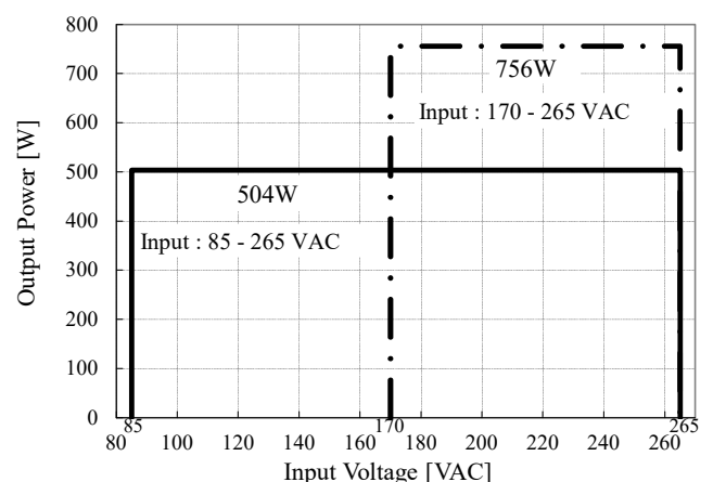
PF500A-360 Derating Curve at Baseplate Temperature = 85°C
