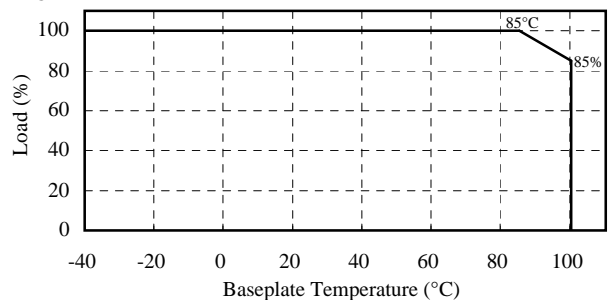
Derating Curve
