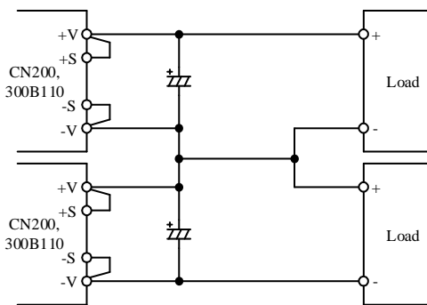
Fig.7-21 ±Output Series Operation
