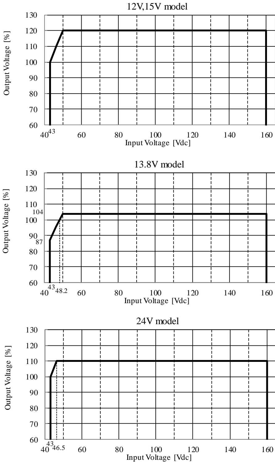
Fig.7-2 Limit of Input voltage
