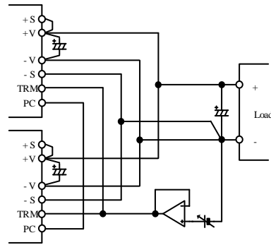
Fig.7-19 Variable Output Voltage (by Applied External Voltage)
