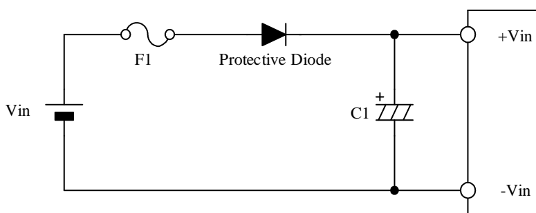
Fig.6-3 Series Connected Input Diode Application
