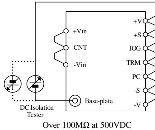
Fig.7-29 Isolation Resistance Test
