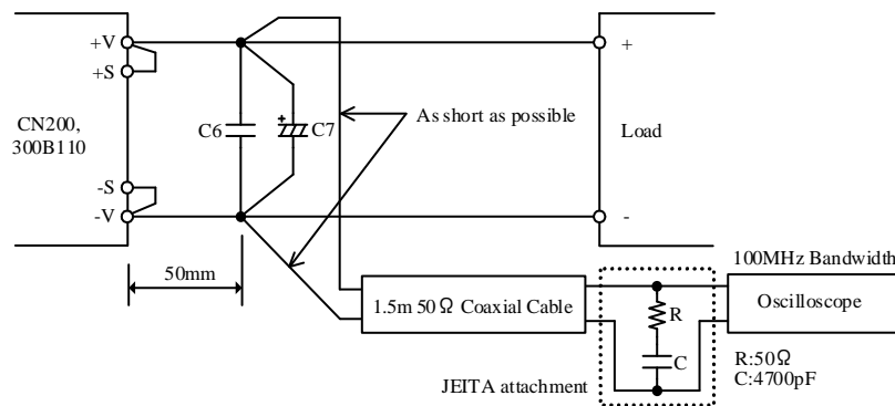
Fig.7-11 Measurement of Maximum Output Ripple and Noise
