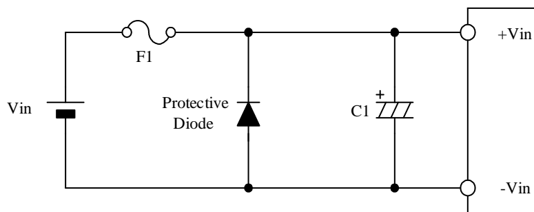
Fig.6-2 Protection for Reversed Connection of Input
