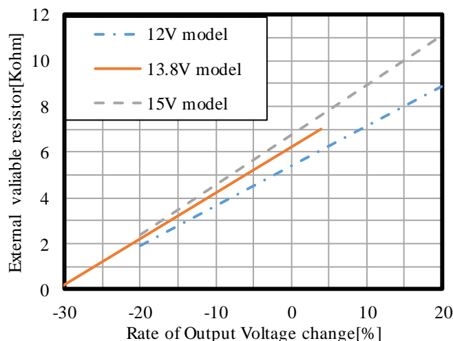
Fig.7-8 External Variable Resistor(VR) vs. Δ(%)
