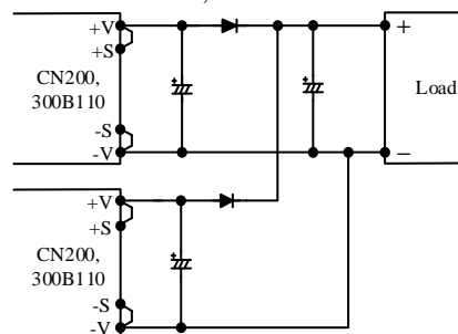
Fig.7-22 Redundant Operation Connection
