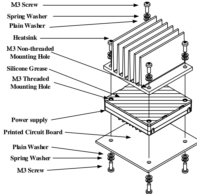
(a) Standard Mounting Method
