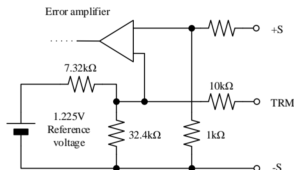
Fig.7-10 Internal TRM circuit (for the reference)
