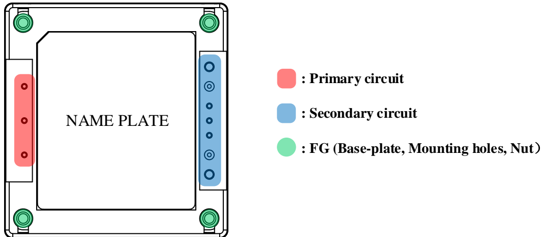
Fig.8-2 Connection potential of each terminal
