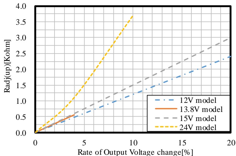
Fig.7-6 Radj(up) vs. Δ(%)
