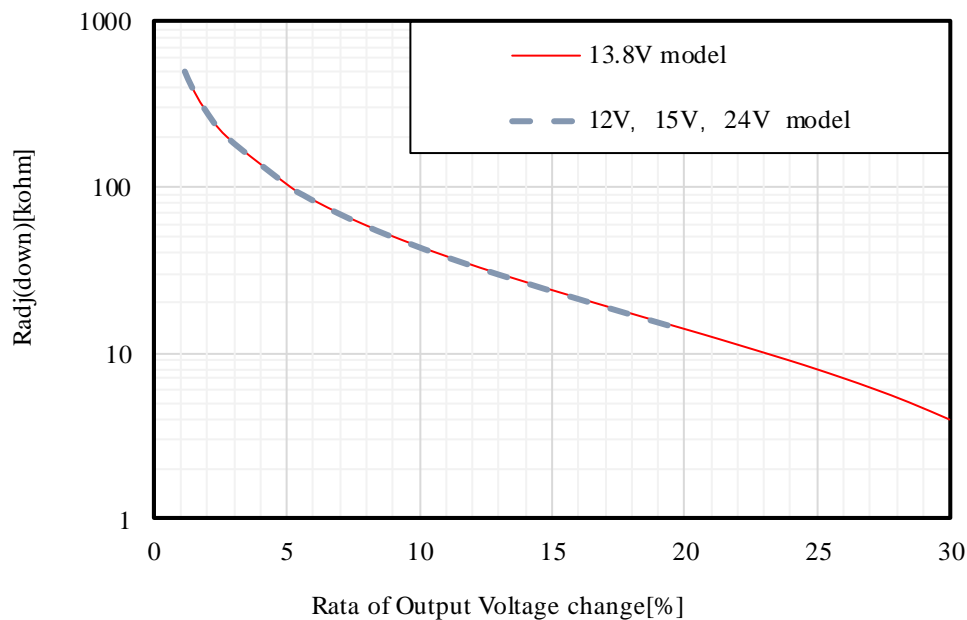
Fig.7-4 Radj(down) vs. \Delta(\%)
