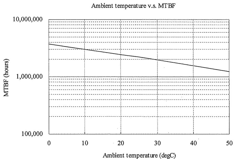
— PSD6-48-1212 Load 100%
