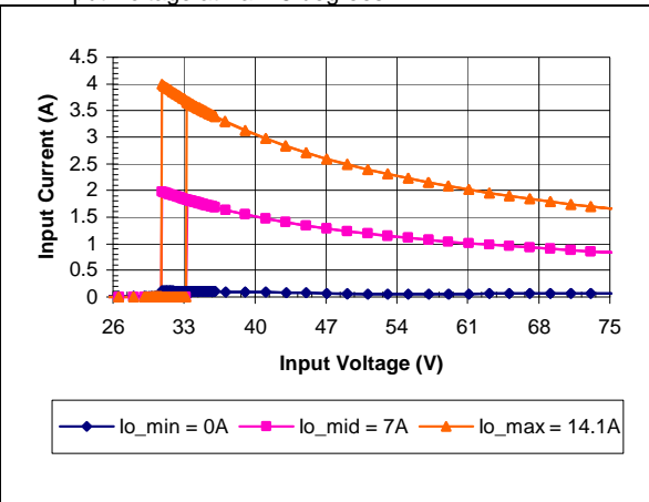
iQE48014A080V-001 Typical Input Current vs. Input Voltage Characteristics
