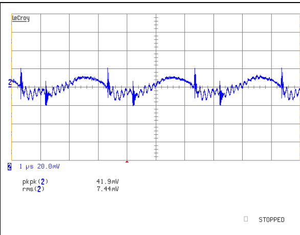
iQE48014A080V-001 Typical Output Ripple at nominal Input voltage and full load at Ta=25 degree
