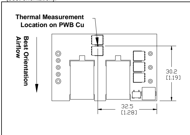
iQE48040A033V-001 thermal measurement location – top view
