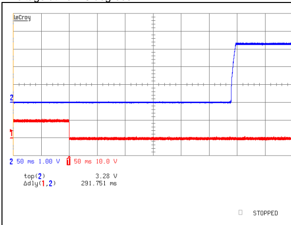
iQE48040A033V-001 Typical startup characteristic from on/off at full load. Lower trace - on/off signal, upper trace – output voltage
