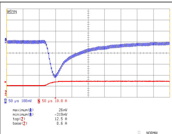
iQE48017A120V-001 Typical transient response. Output voltage response to load step from 50% to 75% of full load with output current slew rate of 0.1A/uS.
