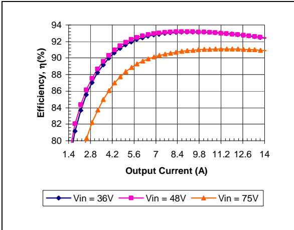
iQE48014A080V-001 Typical Efficiency vs. Input Voltage at Ta=25 degrees.
