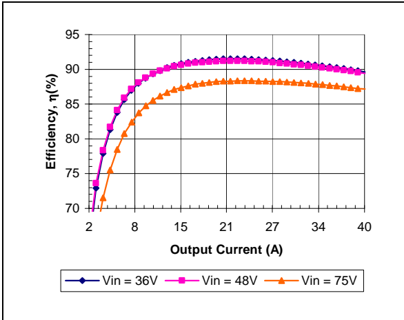
iQE48040A033V-001 Typical Efficiency vs. Input Voltage at Ta=25 degrees.
