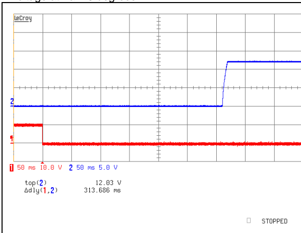
iQE48017A120V-001 Typical startup characteristic from on/off at full load. Lower trace - on/off signal, upper trace – output voltage
