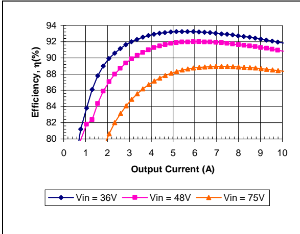
iQE48010A150V-001 Typical Efficiency vs. Input Voltage at Ta=25 degrees.
