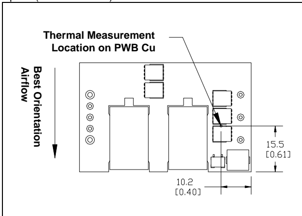
iQE48014A080V-001 thermal measurement location – top view
