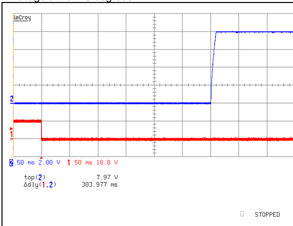
iQE48014A080V-001 Typical startup characteristic from on/off at full load. Lower trace - on/off signal, upper trace – output voltage
