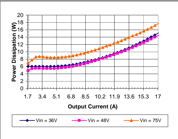
iQE48017A120V-001 Typical Power Dissipation vs. Input Voltage at Ta=25 degrees
