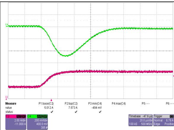
iQE48010A150V-001 Typical transient response. Output voltage response to load step from 50% to 75% of full load with output current slew rate of 0.1A/uS.
