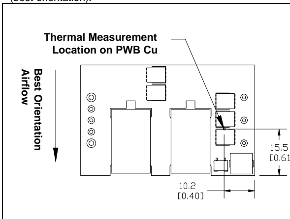
iQE48010A150V-001 thermal measurement location – top view
