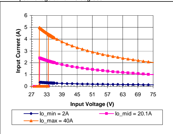
iQE48040A033V-001 Typical Input Current vs. Input Voltage Characteristics
