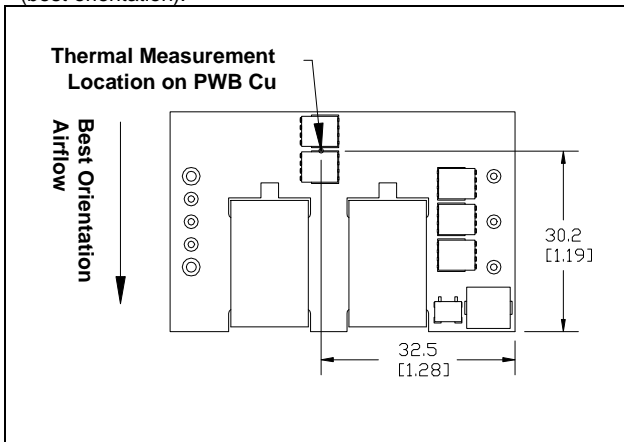
iQE48030A050V-001 thermal measurement location – top view
