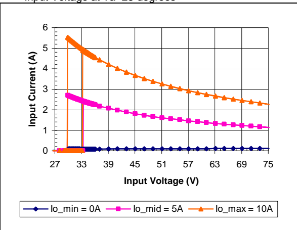
iQE48010A150V-001 Typical Input Current vs. Input Voltage Characteristics
