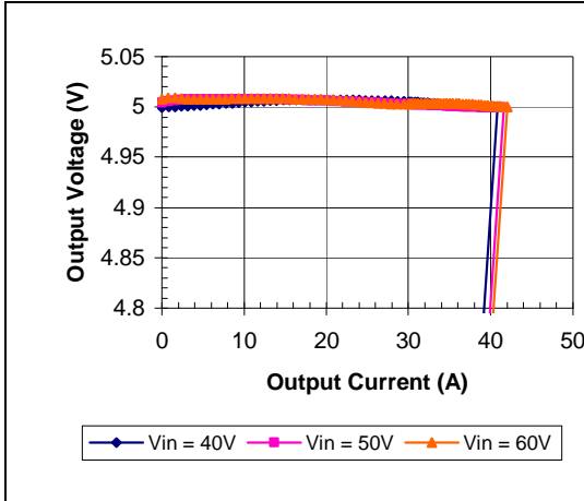
iQE48030A050V-001 Typical Output Current Limit Characteristics vs. Input Voltage at Ta=25 degrees.
