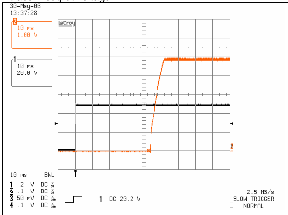
iQE48030A050V-001 Typical startup characteristic from input voltage application at full load. Upper trace - output voltage, lower trace –input voltage
