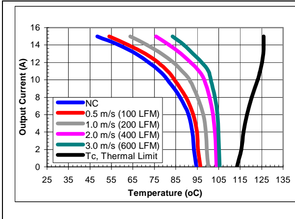
iQE48014A080V-001 preliminary maximum output current vs. ambient temperature at nominal input voltage for airflow rates natural convection (60lfm) to 600lfm with airflow from pin 3 to pin 1 (best orientation).
