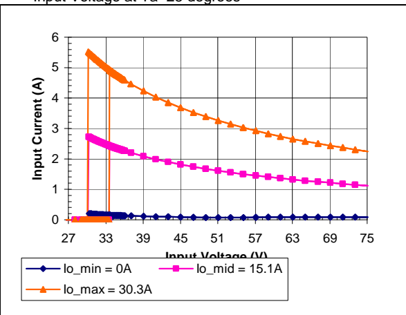
iQE48030A050V-001 Typical Input Current vs. Input Voltage Characteristics
