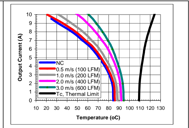
iQE48010A150V-001 maximum output current vs. ambient temperature at nominal input voltage for airflow rates natural convection (60lfm) to 600lfm with airflow from pin 1 to pin 3
