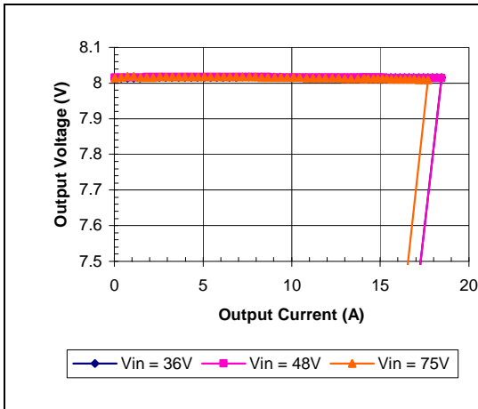
iQE48014A080V-001 Typical Output Current Limit Characteristics vs. Input Voltage at Ta=25 degrees.
