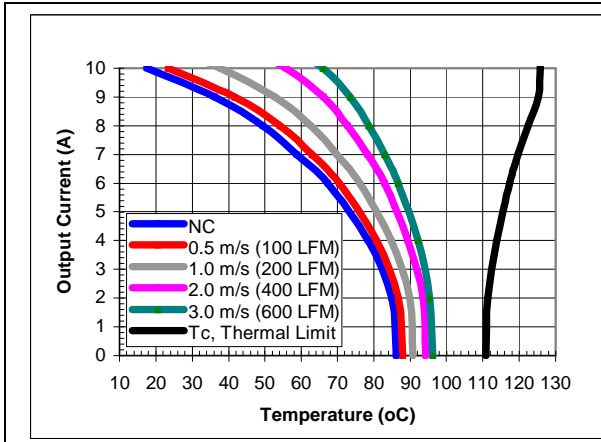
iQE48010A150V-001 maximum output current vs. ambient temperature at nominal input voltage for airflow rates natural convection (60lfm) to 600lfm with airflow from pin 3 to pin 1 (best orientation).
