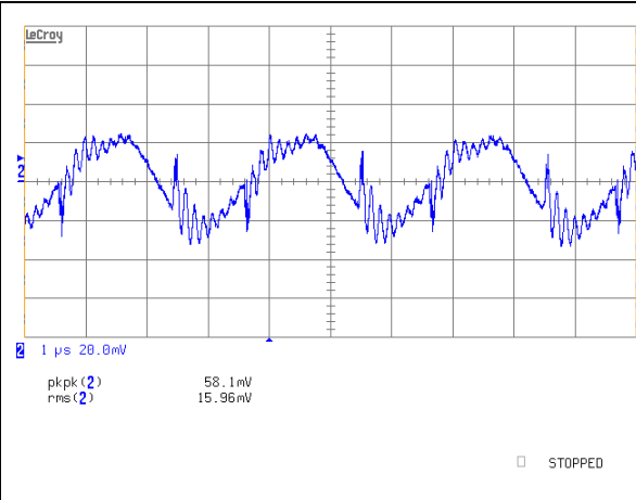
iQE48040A033V-001 Typical Output Ripple at nominal Input voltage and full load at Ta=25 degree
