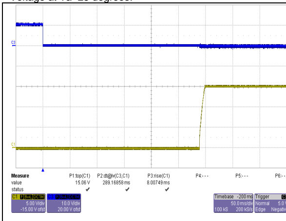
iQE48010A150V-001 Typical startup characteristic from on/off at full load. Lower trace - on/off signal, upper trace – output voltage
