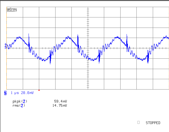
iQE48017A120V-001 Typical Output Ripple at nominal Input voltage and full load at Ta=25 degree
