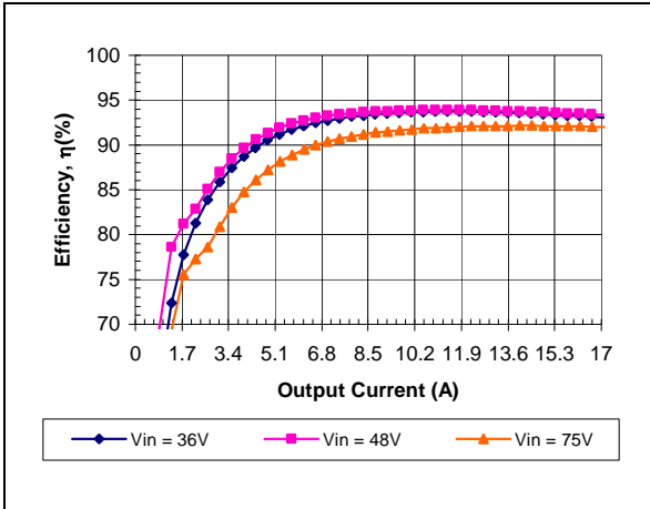
iQE48017A120V-001 Typical Efficiency vs. Input Voltage at Ta=25 degrees.
