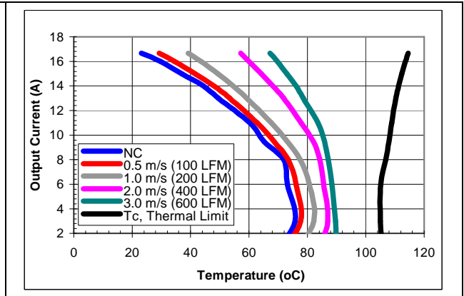
iQE48017A120V-001 maximum output current vs. ambient temperature at nominal input voltage for airflow rates natural convection (60lfm) to 600lfm with airflow from pin 1 to pin 3
