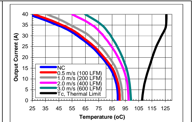
iQE48040A033V-001 maximum output current vs. ambient temperature at nominal input voltage for airflow rates natural convection (60lfm) to 600lfm with airflow from pin 1 to pin 3
