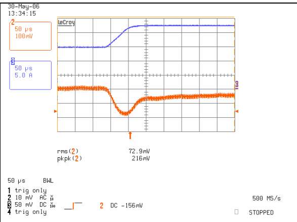
iQE48030A050V-001 Typical transient response. Output voltage response to load step from 50% to 75% of full load with output current slew rate of 0.1A/uS.
