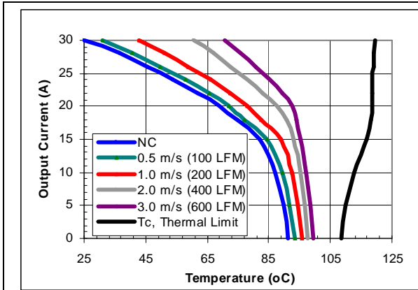
iQE48030A050V-001 maximum output current vs. ambient temperature at nominal input voltage for airflow rates natural convection (60lfm) to 600lfm with airflow from pin 3 to pin 1 (best orientation).
