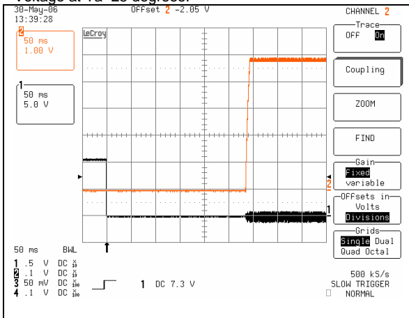
iQE48030A050V-001 Typical startup characteristic from on/off at full load. Lower trace - on/off signal, upper trace – output voltage
