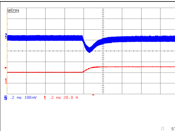
iQE48040A033V-001 Typical transient response. Output voltage response to load step from 50% to 75% of full load with output current slew rate of 0.1A/uS.
