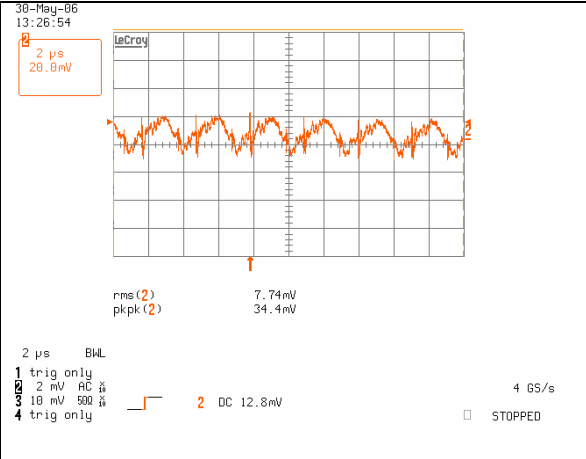
iQE48030A050V-001 Typical Output Ripple at nominal Input voltage and full load at Ta=25 degree
