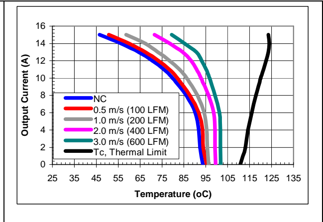
iQE48014A080V-001 maximum output current vs. ambient temperature at nominal input voltage for airflow rates natural convection (60lfm) to 600lfm with airflow from pin 1 to pin 3
