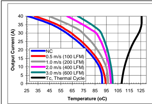
iQE48040A033V-001 maximum output current vs. ambient temperature at nominal input voltage for airflow rates natural convection (60lfm) to 600lfm with airflow from pin 3 to pin 1 (best orientation).
