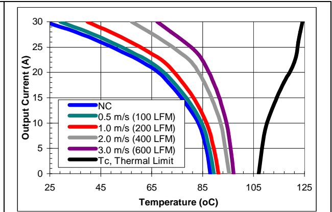
iQE48030A050V-001 maximum output current vs. ambient temperature at nominal input voltage for airflow rates natural convection (60lfm) to 600lfm with airflow from pin 1 to pin 3
