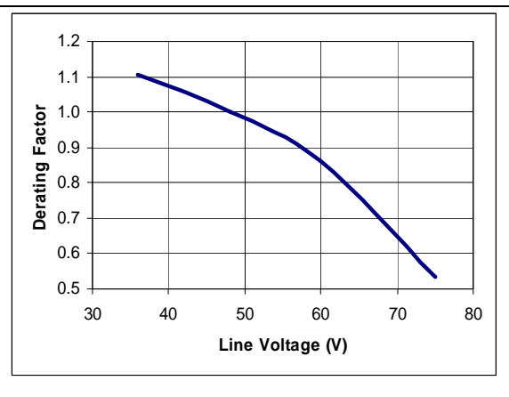
iQE48010A150V-001 typical ambient temperature derating versus line voltage at 200lfm with airflow 1m/s (200lfm)
