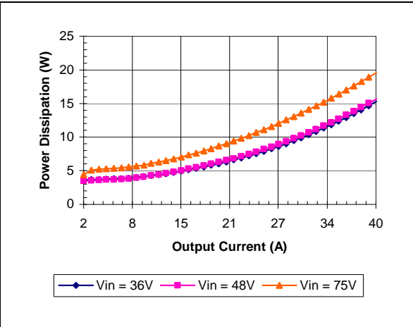
iQE48040A033V-001 Typical Power Dissipation vs. Input Voltage at Ta=25 degrees
