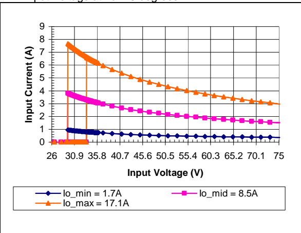
iQE48017A120V-001 Typical Input Current vs. Input Voltage Characteristics
