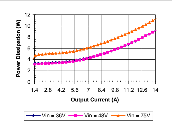
iQE48014A080V-001 Typical Power Dissipation vs. Input Voltage at Ta=25 degrees
