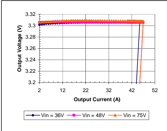
iQE48040A033V-001 Typical Output Current Limit Characteristics vs. Input Voltage at Ta=25 degrees.
