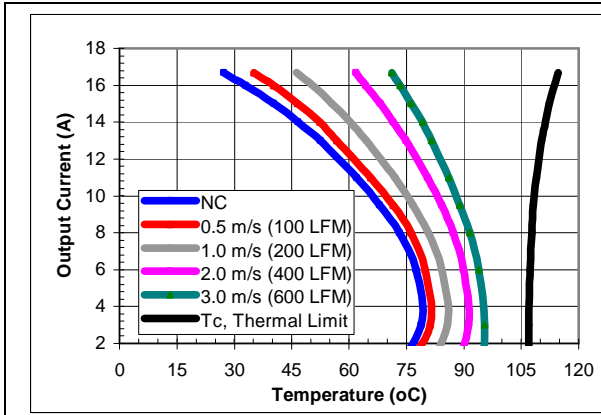
iQE48017A120V-001 maximum output current vs. ambient temperature at nominal input voltage for airflow rates natural convection (60lfm) to 600lfm with airflow from pin 3 to pin 1 (best orientation).
