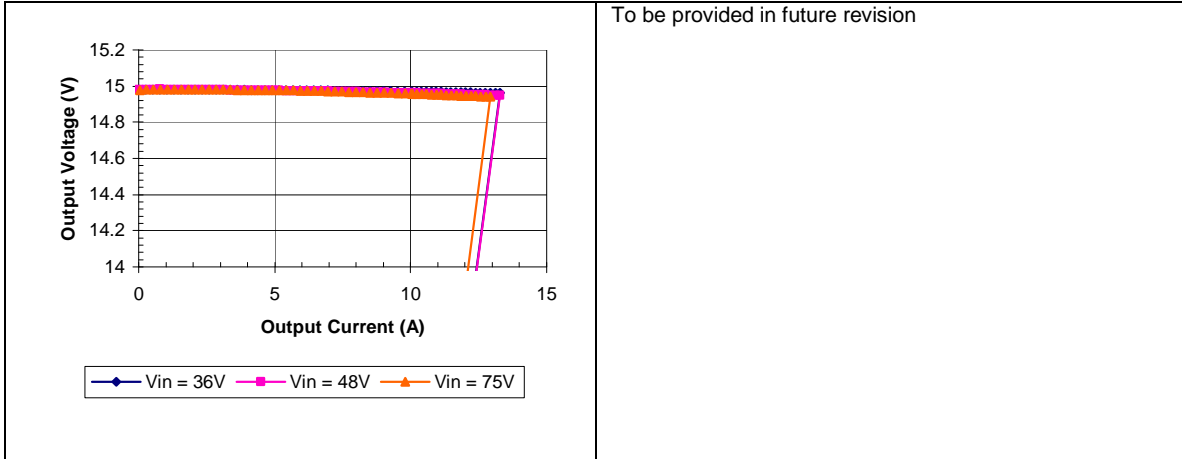
iQE48010A150V-001 Typical Output Current Limit Characteristics vs. Input Voltage at Ta=25 degrees.
