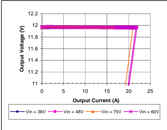
iQE48017A120V-001 Typical Output Current Limit Characteristics vs. Input Voltage at Ta=25 degrees.
