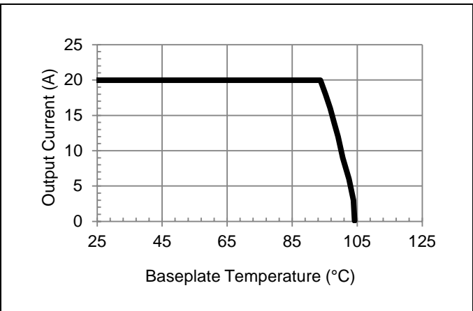
V_o = 12\text{ V} , V_{in} = 48\text{ V} maximum baseplate temperature in conduction cooling applications.
