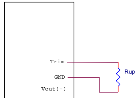
Circuit to increase output voltage
