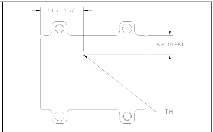
RGA4W250W010A thermal measurement location (Tc) – top view
