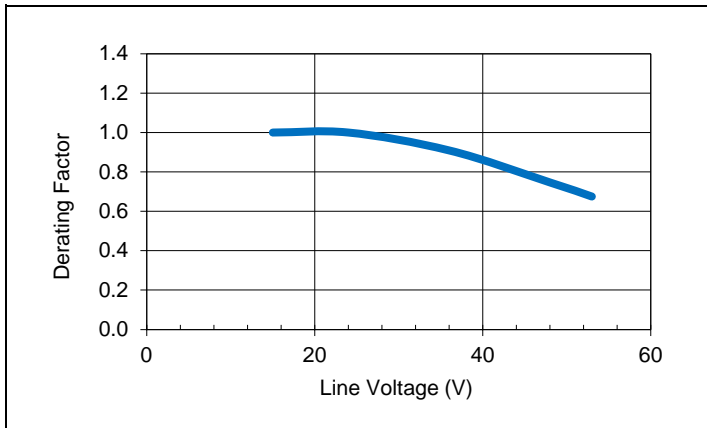
Average output current derating versus line voltage with airflow 1m/s (200 lfm)
