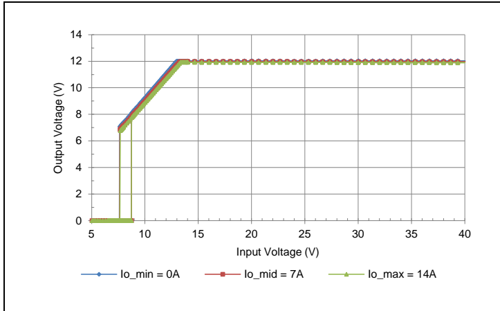
V_o = 12V Typical Output Voltage vs. Input Voltage Characteristics.
