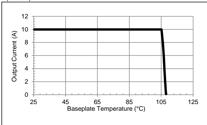
Vo = 12 V, Vin = 24 V maximum baseplate temperature in conduction cooling applications.
