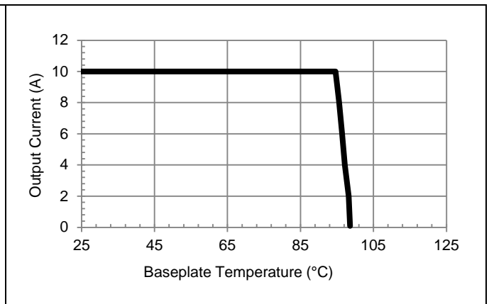
Vo = 12 V, Vin = 48 V maximum baseplate temperature in conduction cooling applications.
