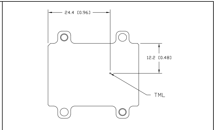
RGA4W250W014A thermal measurement location (Tc) – top view
