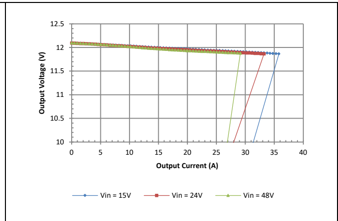
Vo = 12 V Typical Current Limit Characteristic.
