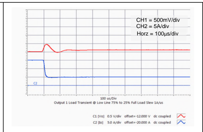
Vo=12 V Typical output voltage transient response to load step from 75% to 25% of full load with output current slew rate of 1 A/µs (Cext = 200 µF).
