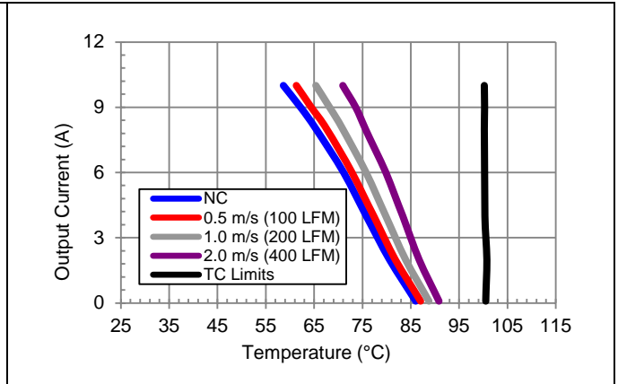
Vo = 12 V, Vin = 48 V preliminary maximum output current vs. ambient temperature at nominal input voltage for natural convection (60lfm) to 400lfm with airflow from pin 8 to pin 4.
