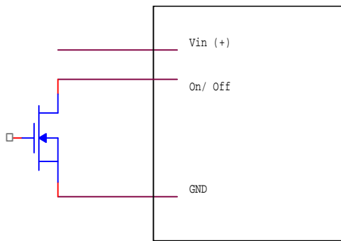
On/Off Circuit for positive or negative logic
