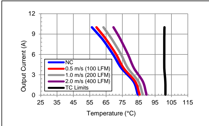
Vo = 24 V, Vin = 48 V preliminary maximum output current vs. ambient temperature at nominal input voltage for natural convection (60lfm) to 400lfm with airflow from pin 8 to pin 4.
