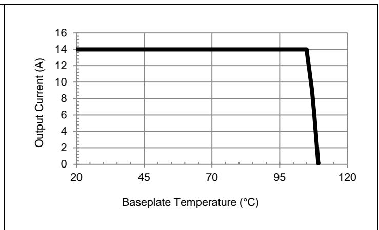
Vo = 3.3 V, Vin = 24 V maximum baseplate temperature in conduction cooling applications.
