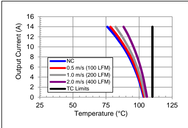
Vo = 18V, Vin = 24V preliminary maximum output current vs. ambient temperature at nominal input voltage for natural convection (60lfm) with airflow from pin 8 to pin 4.
