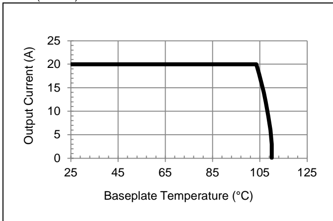
V_o = 12\text{ V} , V_{in} = 24\text{ V} maximum baseplate temperature in conduction cooling applications.
