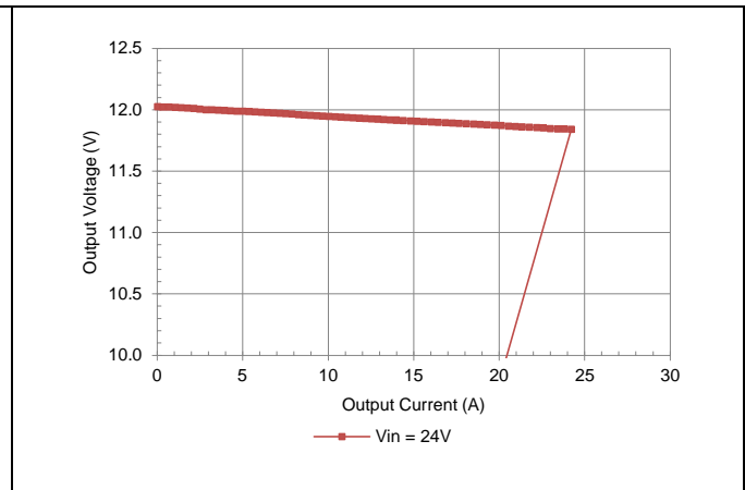
Vo = 12V Typical Current Limit Characteristics.
