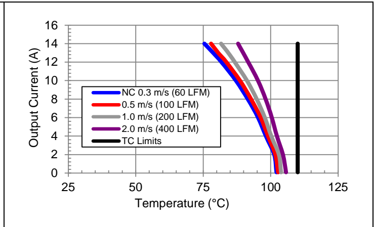
Vo = 12V, Vin = 24V preliminary maximum output current vs. ambient temperature at nominal input voltage for natural convection (60lfm) with airflow from pin 8 to pin 4.
