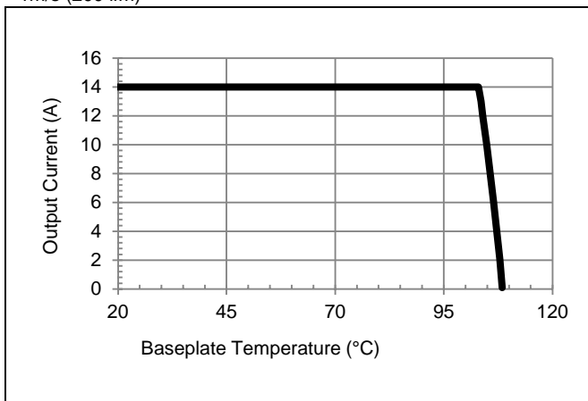
Vo = 18 V, Vin = 24 V maximum baseplate temperature in conduction cooling applications.
