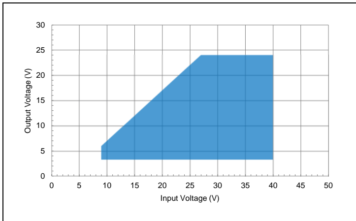
Output Voltage vs. Input Voltage Operating Range.
