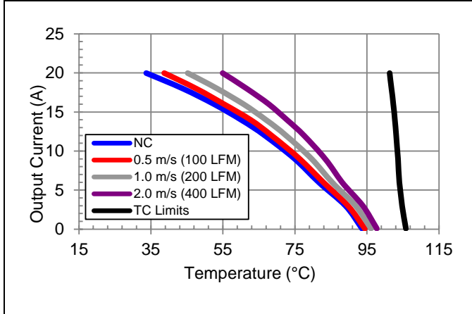
V_o = 5\text{ V} , V_{in} = 48\text{ V} preliminary maximum output current vs. ambient temperature at nominal input voltage for natural convection (60lfm) to 400lfm with airflow from pin 8 to pin 4.
