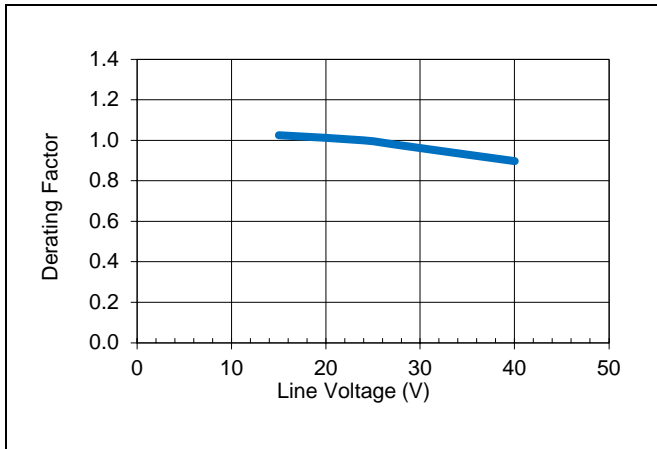
Average output current derating versus line voltage with airflow 1m/s (200 lfm)
