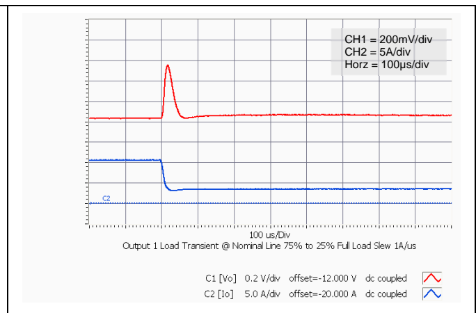
Vo = 12V Typical output voltage transient response to load step from 75% to 25% of full load with output current slew rate of 1A/µs (Cext = 3 x 47µF ceramic capacitor).
