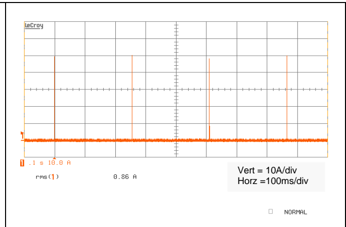
Typical Output Short Circuit Current – CH1, orange.
