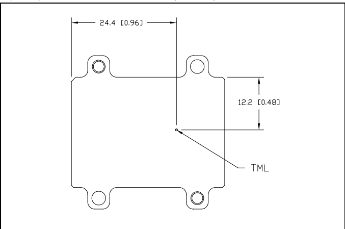
RGA4W250W020A thermal measurement location ( T_c ) – top view
