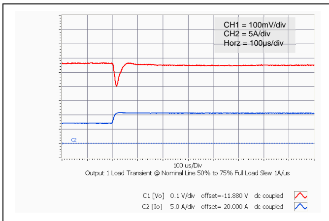
Vo = 12V Typical output voltage transient response to load step from 50% to 75% of full load with output current slew rate of 1A/µs (Cext = 3 x 47µF ceramic capacitor).
