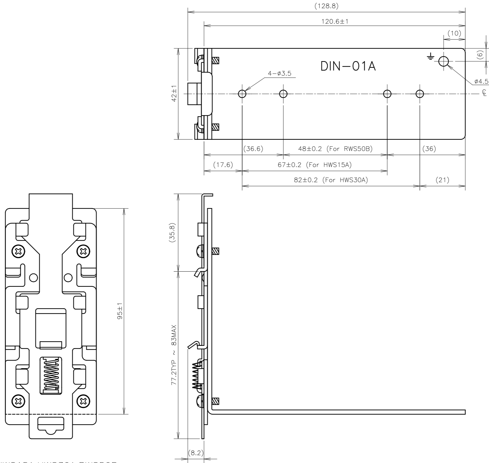
Mounting Plate for HWS15A,HWS30A,RWS50B
