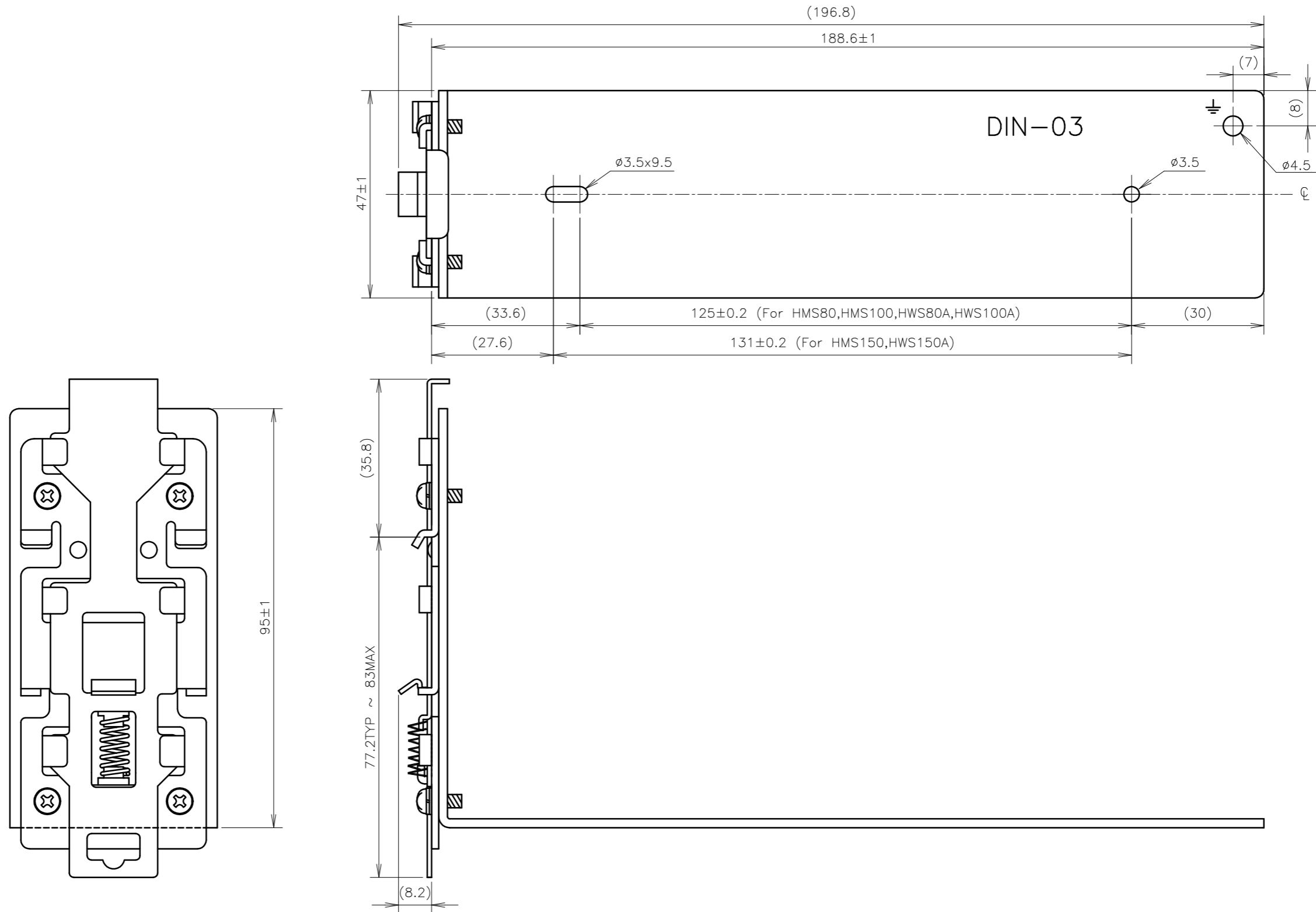
Mounting Plate for HMS80,HMS100,HMS150,HWS80A,HWS100A,HWS150A
